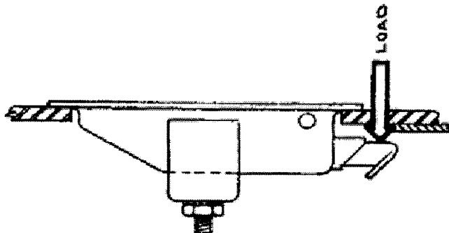
NR 64 PADDLE LATCH - 200 SERIES
