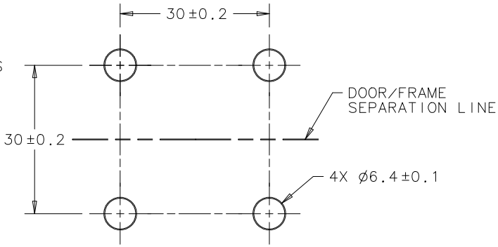
PANEL PREPARATION
