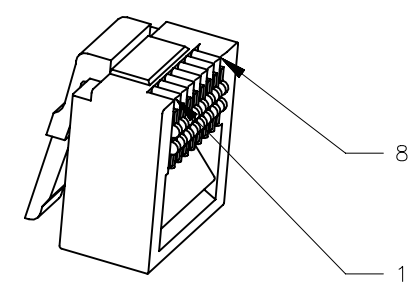
P1 PIN DESIGNATION (2:1 SCALED VIEW)
