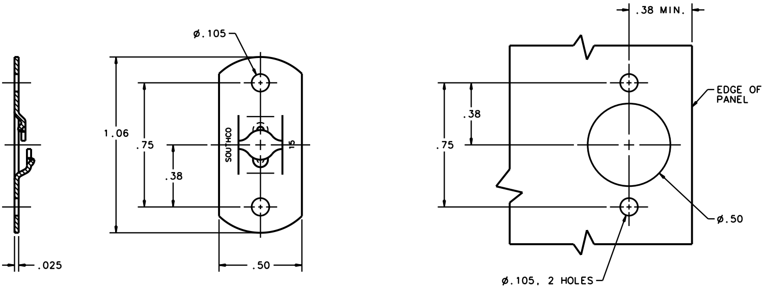
PANEL PREPARATION
