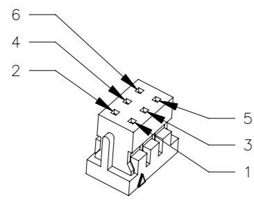
P1 PIN DESIGNATION (2:1 SCALED VIEW)
