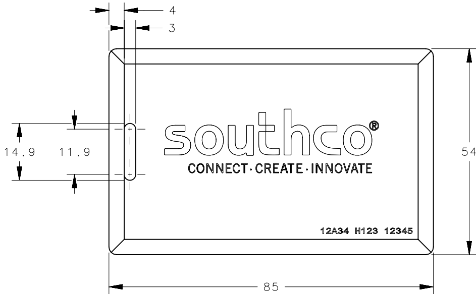
FRONT VIEW (PART NUMBER EA-C2-021-9 SHOWN)
